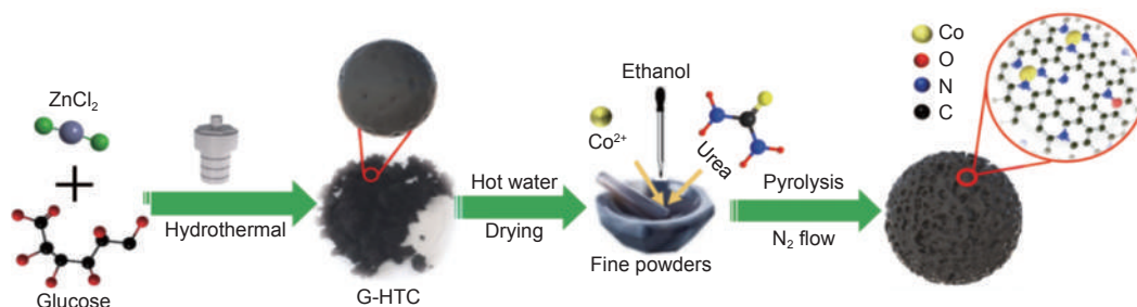
Fig. 1 Schematic diagram for the production of Co–N–C catalysts
