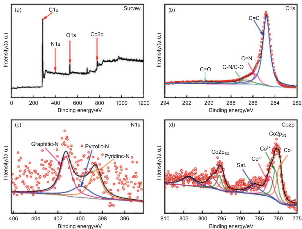
Fig. 6 XPS spectra of 10%Co@NCG-800: (a) survey curve, and high resolution XPS: (b) C1s, (c) N1s and (d) Co2p
