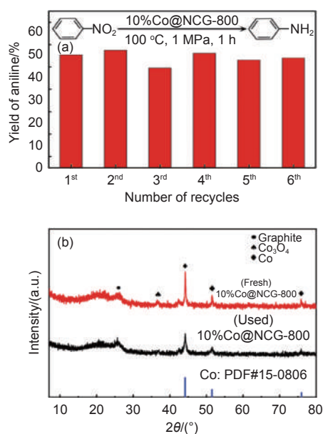
Fig. 8 (a) The reusability of 10%Co@NCG-800 and (b) XRD patterns for the fresh and used catalysts
