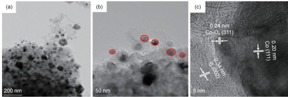
Fig. 3 Typical TEM images for 10%Co@NCG-800 under varied magnifications
