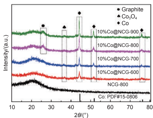
Fig. 5 XRD patterns for the series of catalysts
