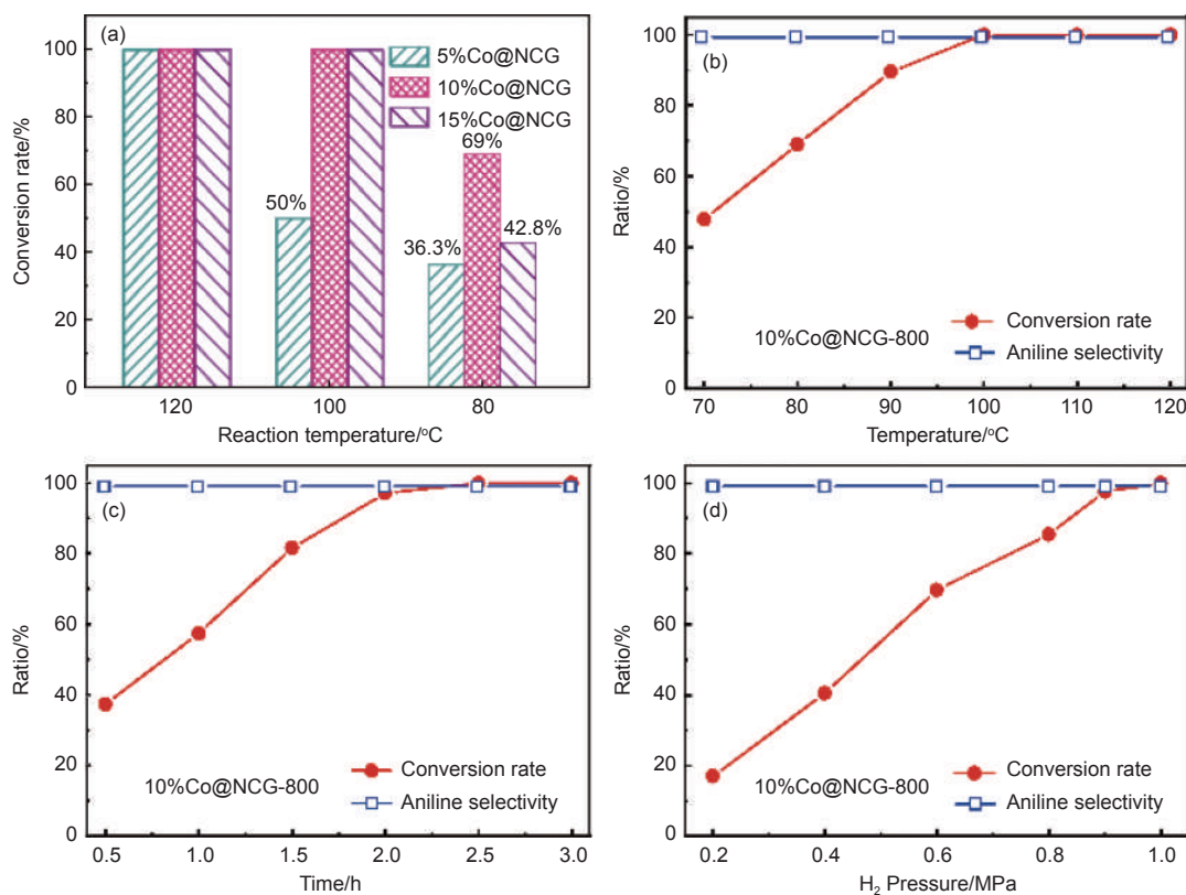
Fig. 7 (a) NB conversion on catalysts as pyrolyzed at 800 °C, and the effects of different reaction parameters on activity over 10%Co@NCG-800 catalyst: (b) temperature, (c) time and (d) H 2 pressure
