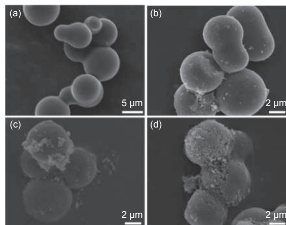
Fig. 2 SEM images for different catalysts: (a) G-HTC, (b) 10%Co@NCG-700, (c) 10%Co@NCG-800 and (d) 10%Co@NCG-900
