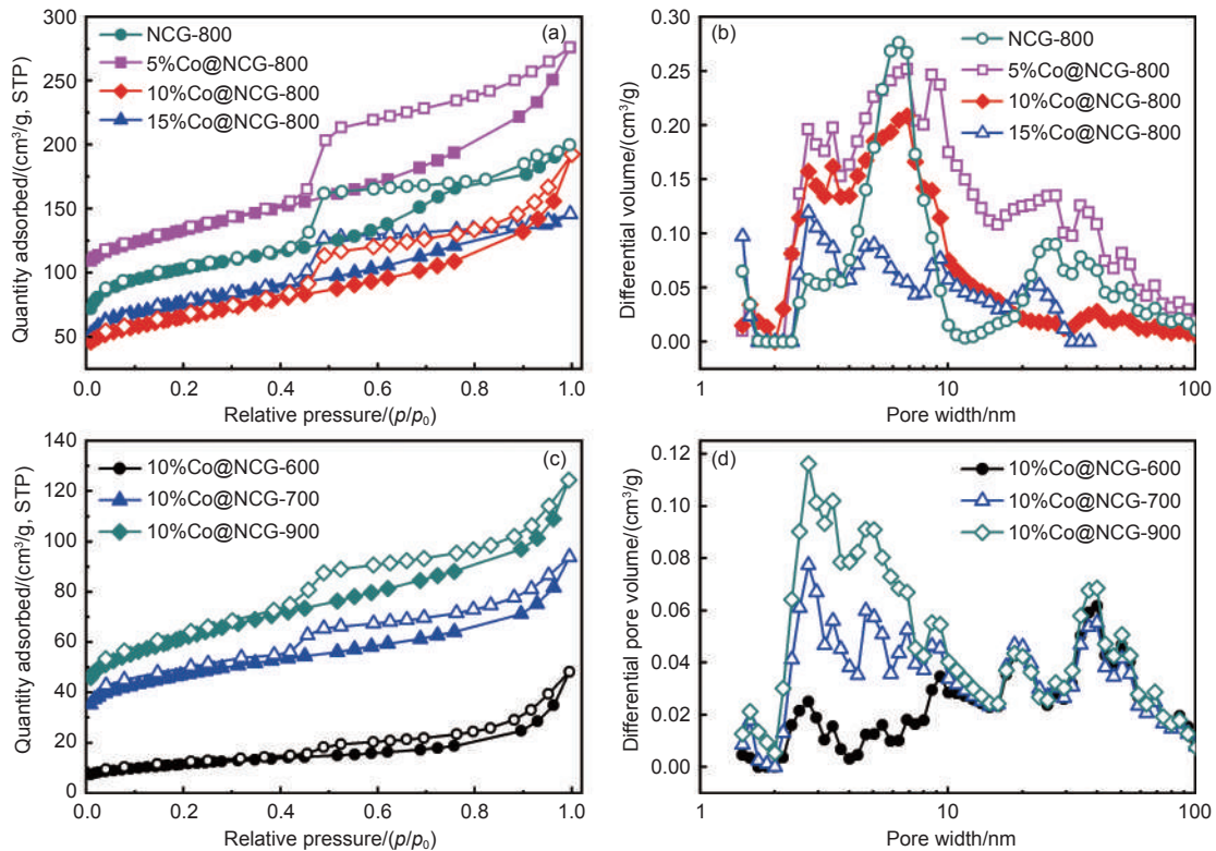
Fig. 4 (a, c) \text{N}_2 isotherms and (b, d) PSDs, and isotherms in Fig. 4a were separately shifted up by 30 \text{ cm}^3/\text{g} for shake of clarity
